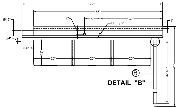
FRONT ELEVATION
